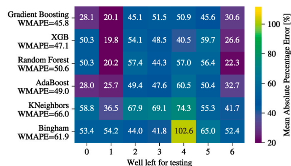
(b) Weighted Mean Absolute Percentage Error
